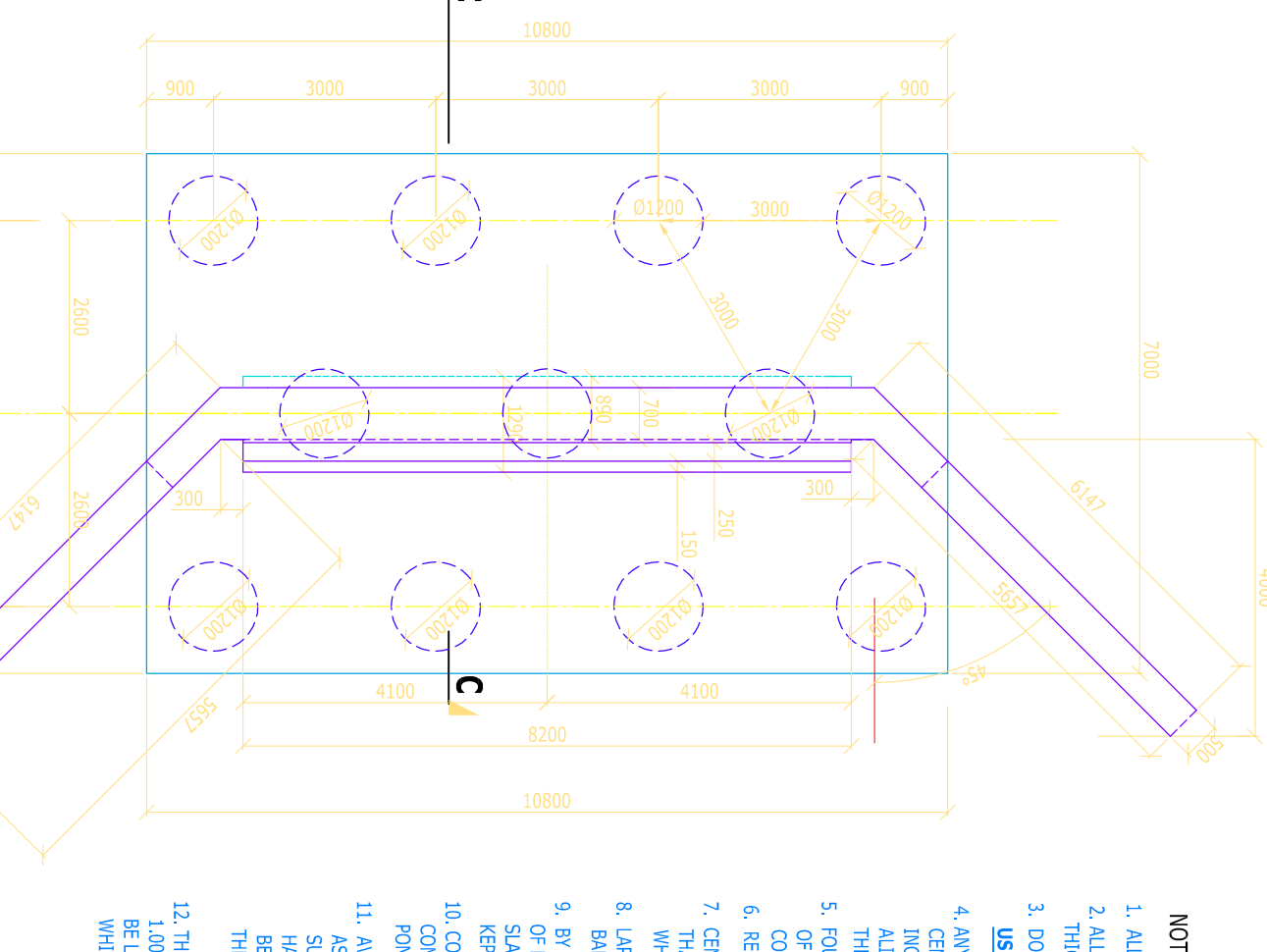
DETAIL FOUNDATION OF ABUTMENT FOR TENDER PURPOSE ONLY
